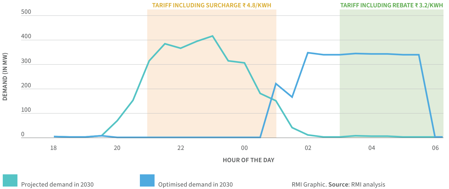
Exhibit 27 Potential of managed charging of e-buses in Delhi in 2030
