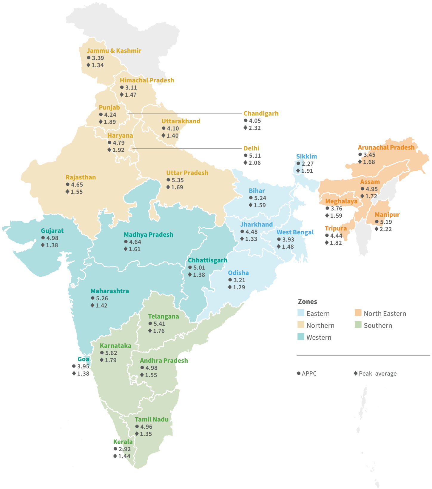
Comparison of peakiness of electricity demand and average power purchase cost (APPC) across all Indian states for fiscal year (FY) 2022
