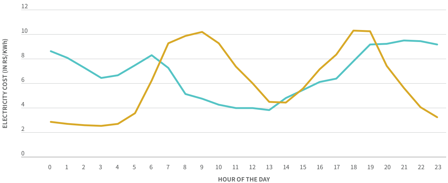
Exhibit 16 Average hourly pricing on the DAM
