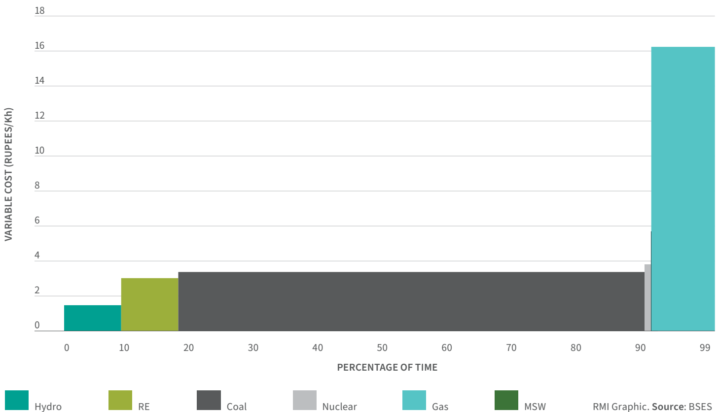
Exhibit 14 Merit order stack of BSES' generators
