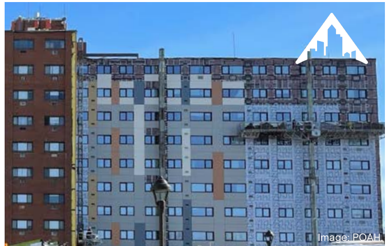
Salem Heights Apartments being wrapped in a new super-insulated shell.
