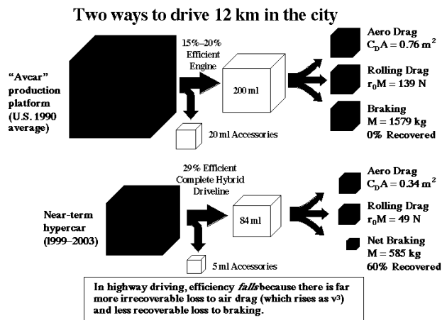
Figure 2 Early hypercars' schematic physical principles
