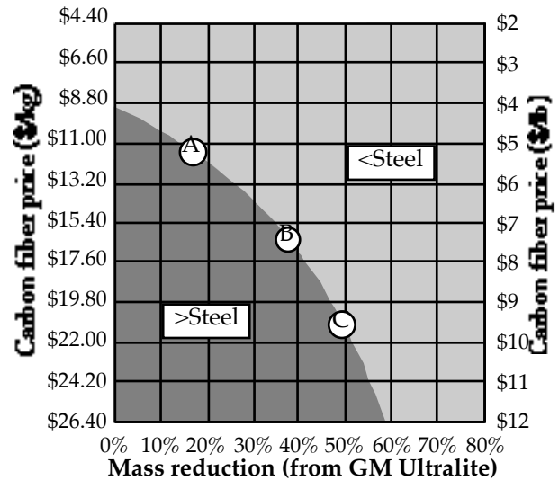
Figure 4 Carbon fiber competes via optimized mass
