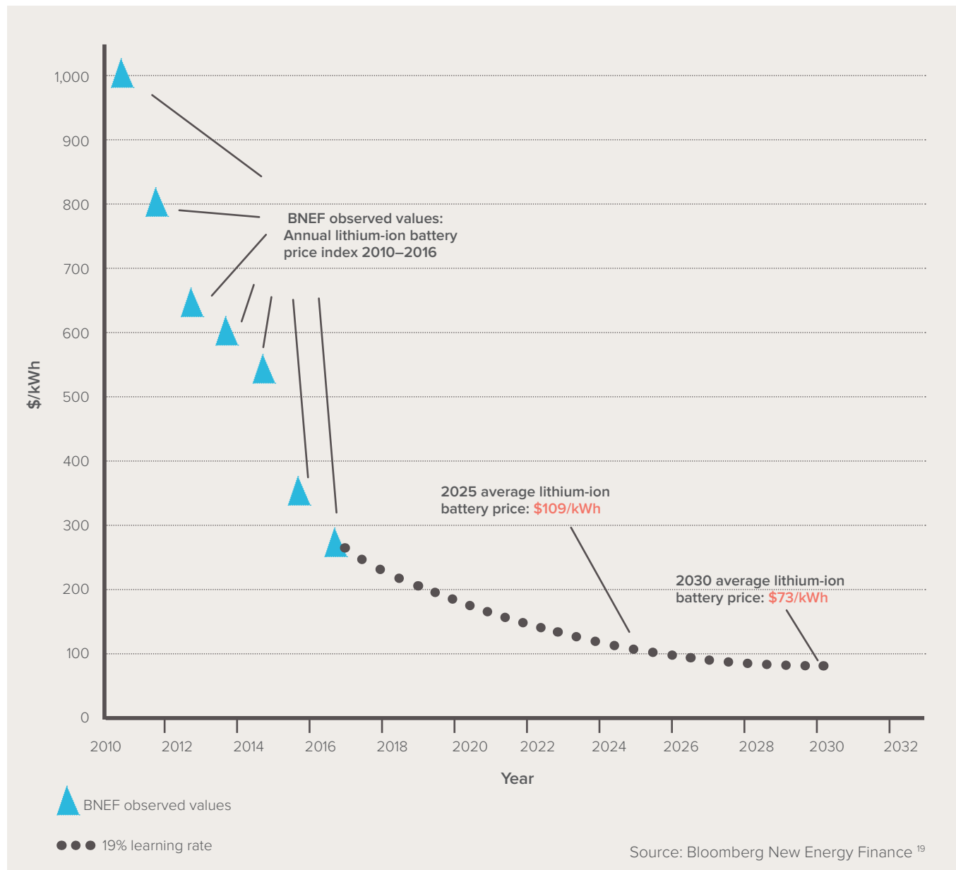
FIGURE 5 BNEF FORECAST FOR THE COMBINED COST OF LITHIUM-ION BATTERY CELLS AND PACKS
