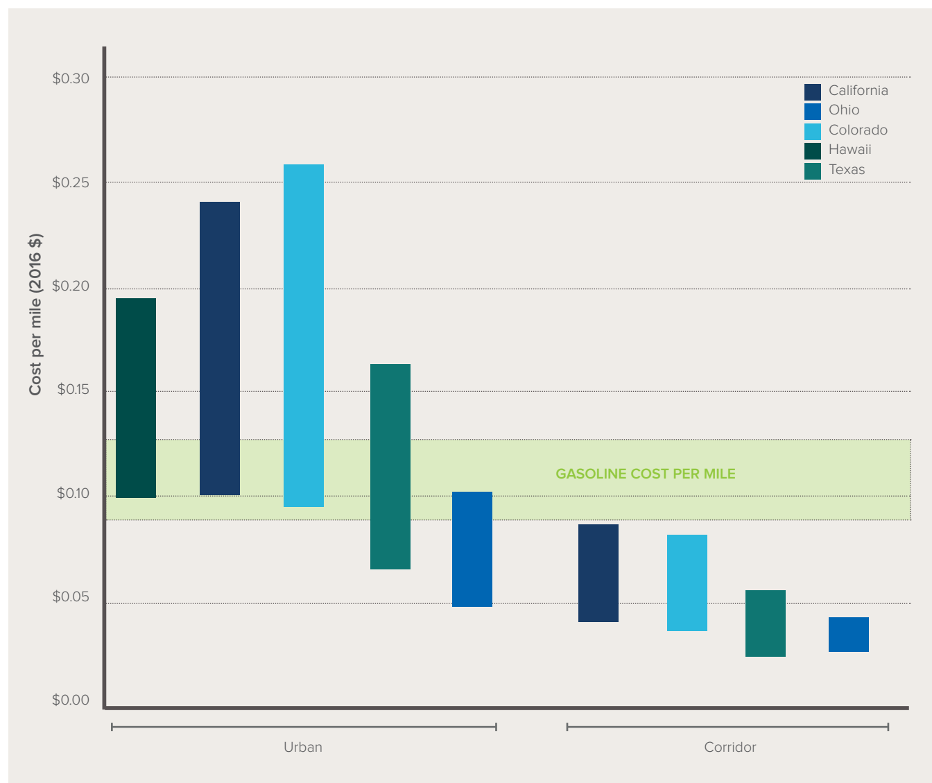
FIGURE 13 ELECTRICITY COST RANGE FOR HOST SITE TO DELIVER ONE MILE OF CHARGE VIA DCFC
