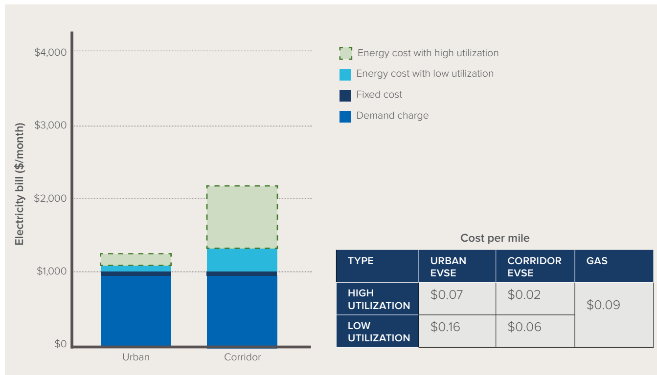
UTILITY BILL FOR A REPRESENTATIVE DCFC IN TEXAS ON THE AUSTIN ENERGY GRID
