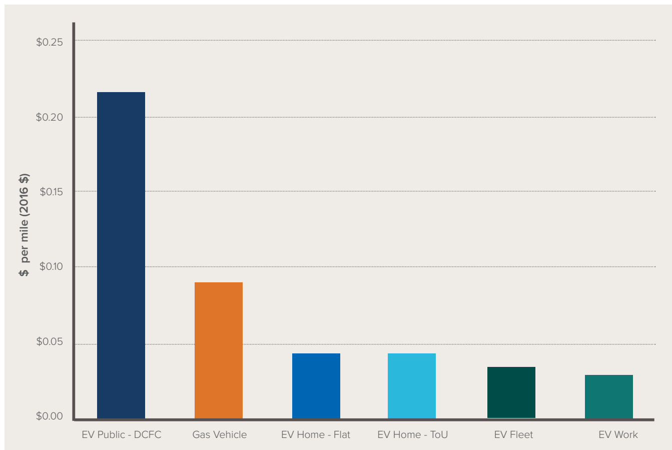
FIGURE 18: EV CHARGING COSTS IN OHIO ON THE AEP GRID
