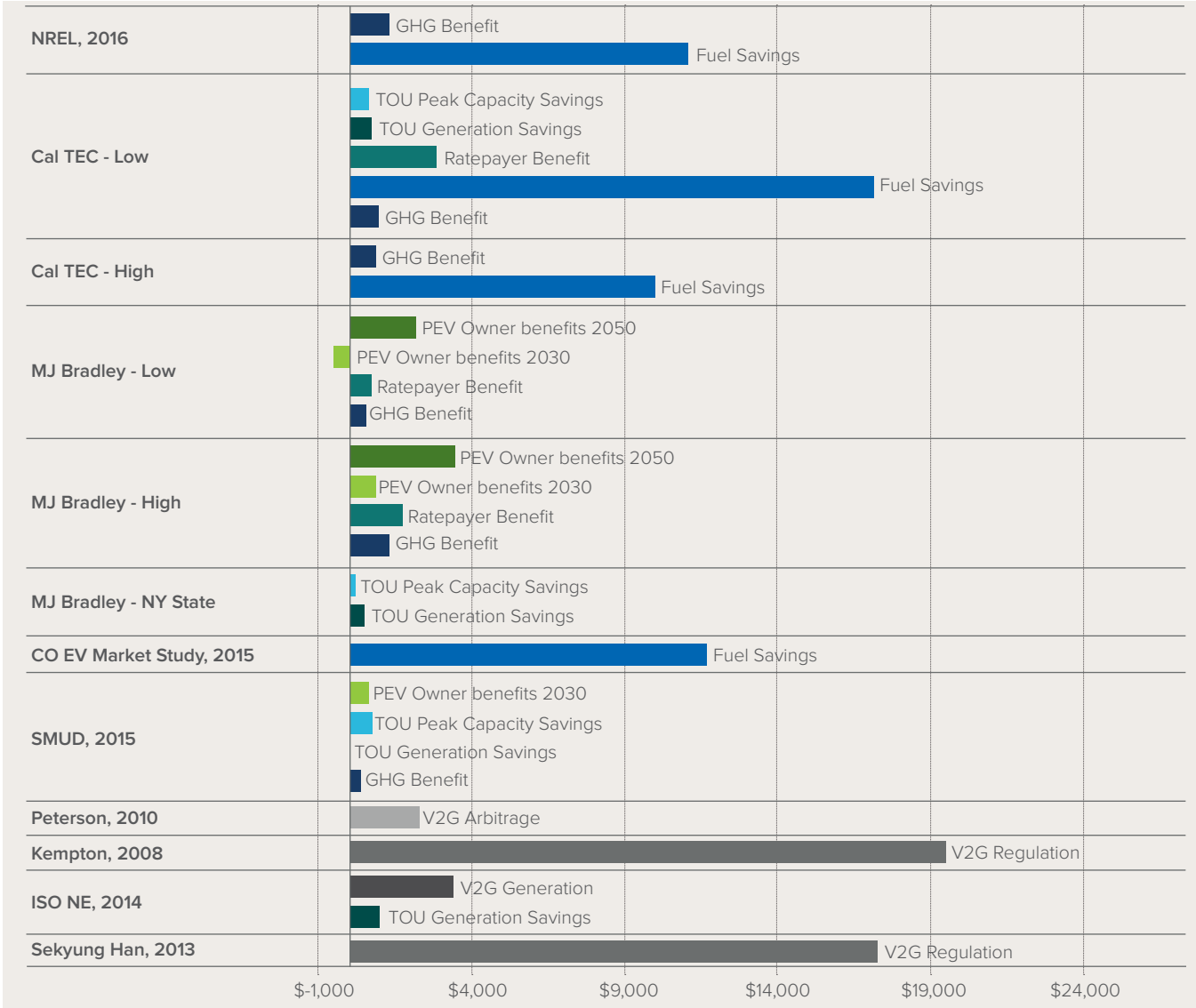
FIGURE 26 DETAIL OF STAKEHOLDER BENEFITS FOR EVS FROM THE LITERATURE
