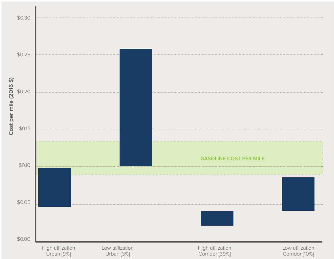
ELECTRICITY COST FOR HOST SITE TO DELIVER ONE MILE OF CHARGE VIA DCFC
