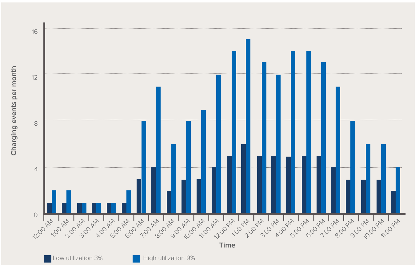
FIGURE 25 URBAN DCFC UTILIZATION PROFILE
