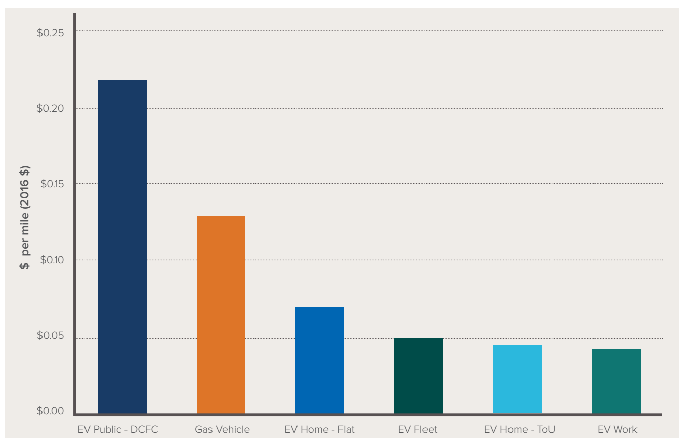
FIGURE 14 EV CHARGING COSTS IN CALIFORNIA, SCE
