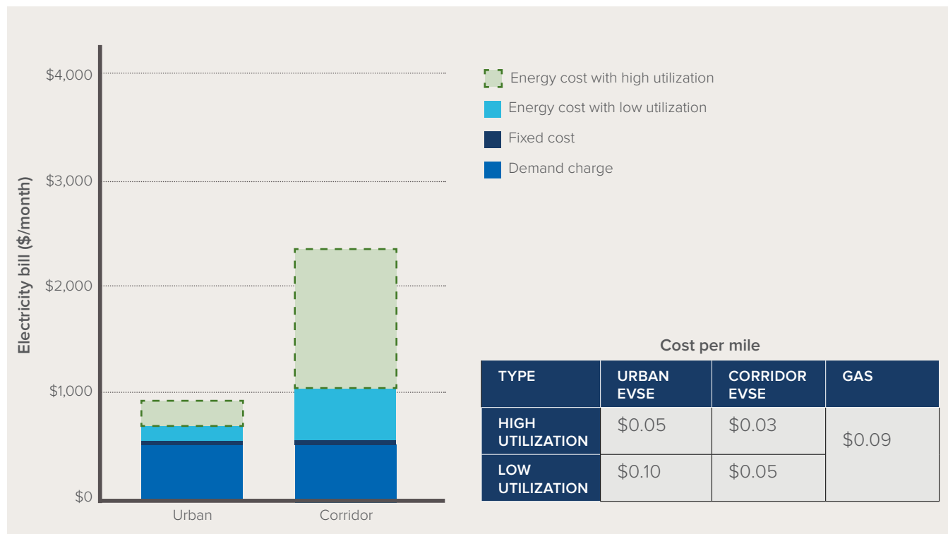
UTILITY BILL FOR A REPRESENTATIVE DCFC IN OHIO ON THE AEP GRID
