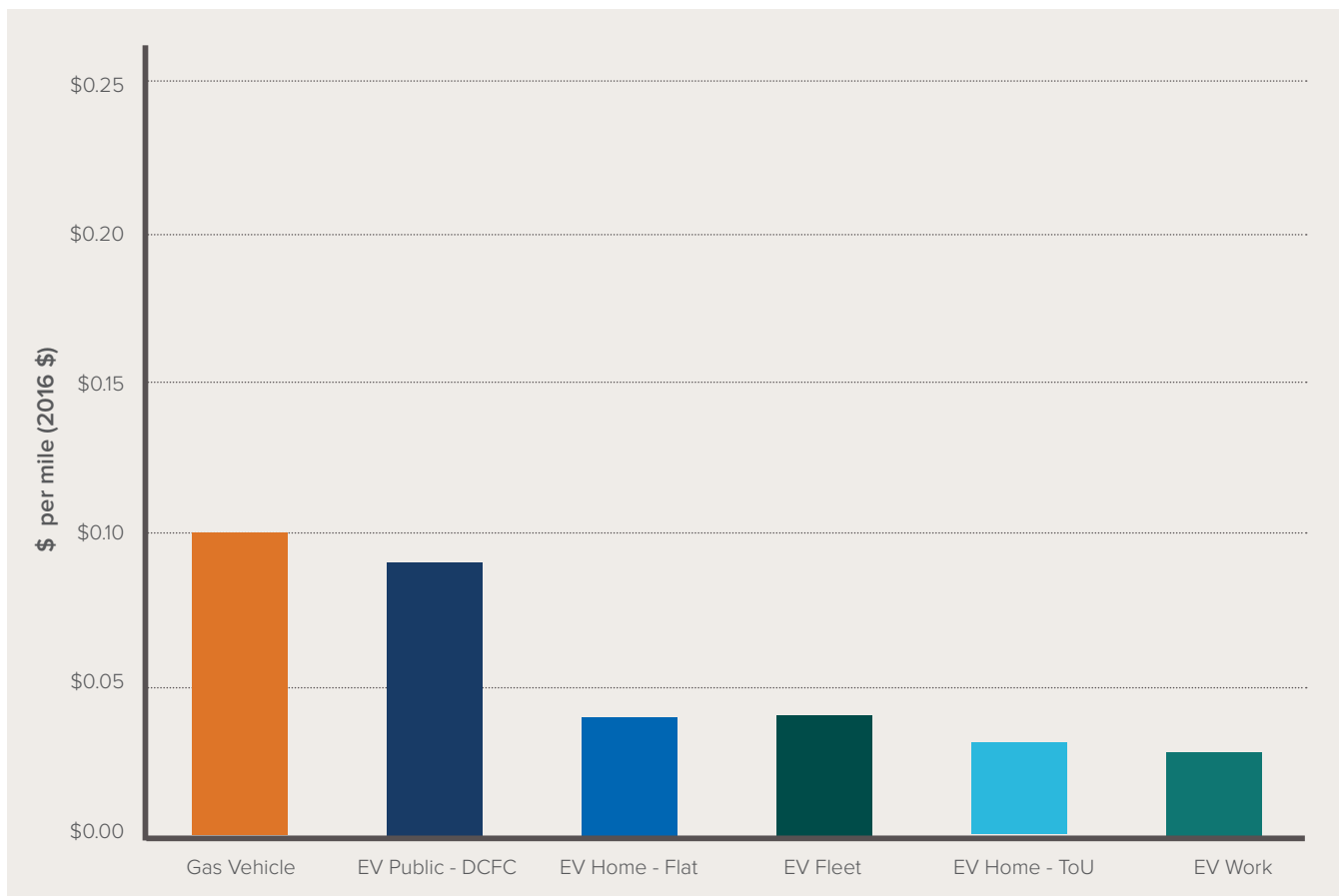
FIGURE 20 EV CHARGING COSTS IN TEXAS ON THE AUSTIN ENERGY GRID
