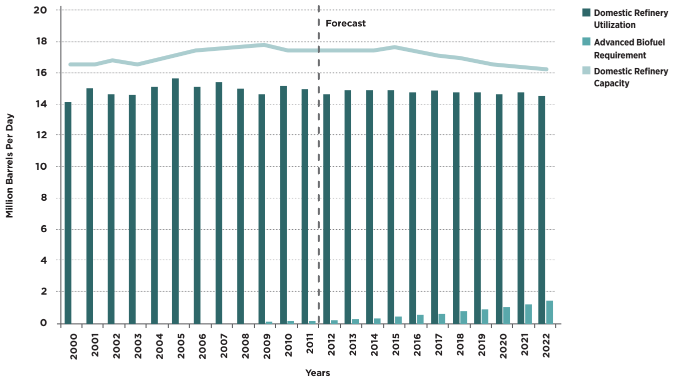
Figure 17: U.S. Domestic Refinery Distillation Capacity, Utilization, and the Advanced Biofuel Requirement
